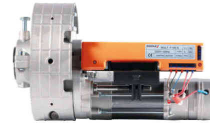
Bolt F Standard model with small control panel
